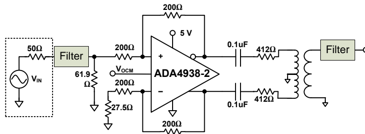
Figure 53. Distortion Measurement Circuit
