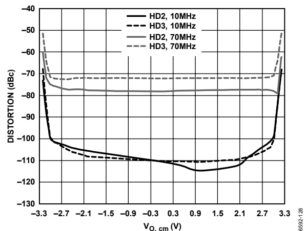
Figure 28. Harmonic Distortion vs. V_{O, cm} and Frequency, V_S = 5V
