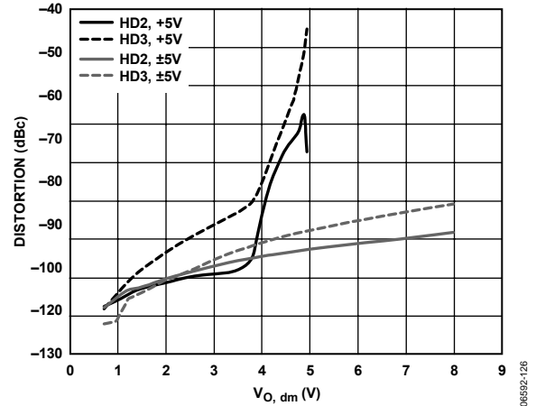
Figure 26. Harmonic Distortion vs. V_{O, dm} and Supply Voltage
